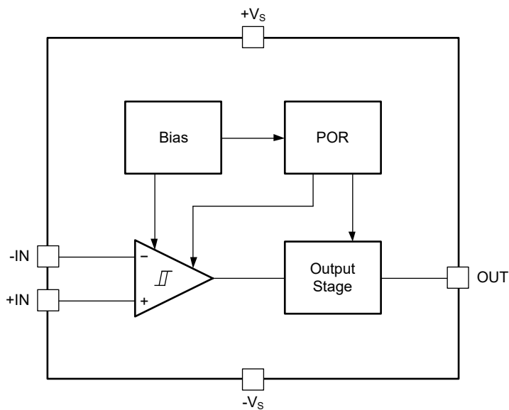
Figure 3. Block Diagram
