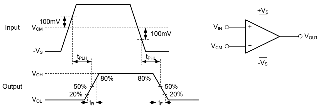
Figure 2. Propagation Delay Diagram
